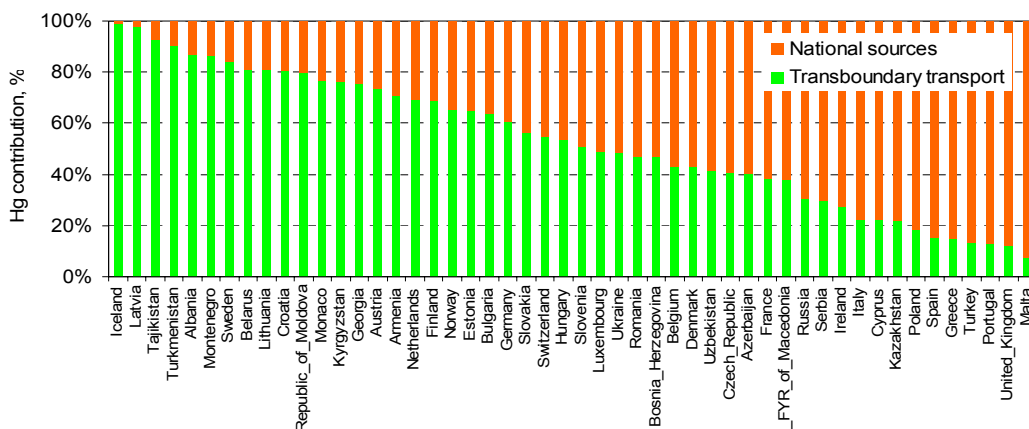
Figure 40. Relative contribution of the transboundary transport and national sources to anthropogenic mercury deposition in the European and Central Asian countries in 2007 (EMEP, 2009b).
