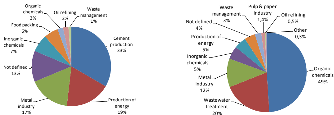
Figure 19. Total loads (main sectors, in %) of mercury to air (left) and water (right), reported by Mediterranean countries in the NBB 2003. Mercury releases to water from the manufacture of fertilizers have been removed.
